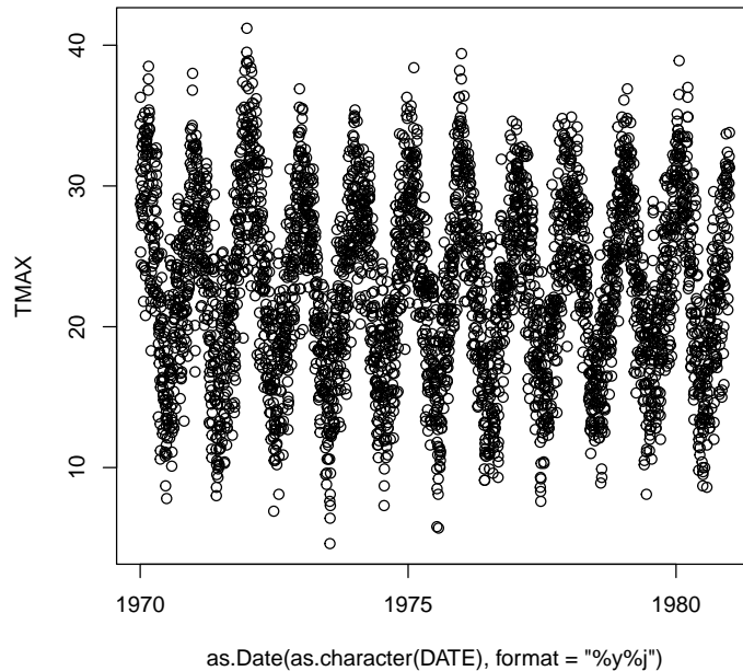
Figure 4: Daily maximum temperature series.
