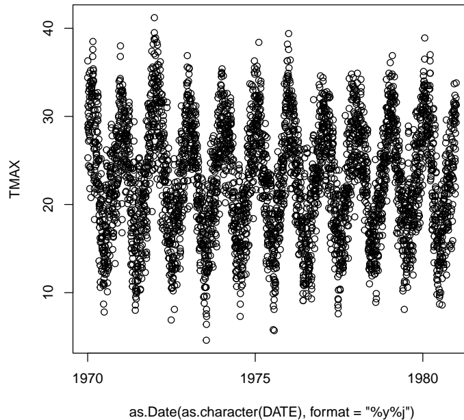
Figure 4: Daily maximum temperature series.
